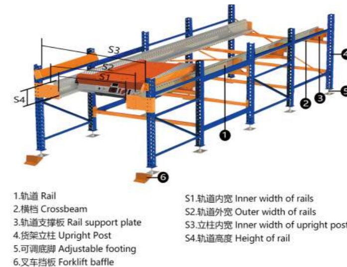
Radio shuttle rack structure details 穿梭式货架结构
