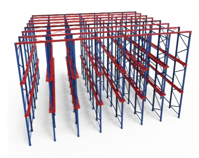
Drive-in rack project 驶入式货架案例
