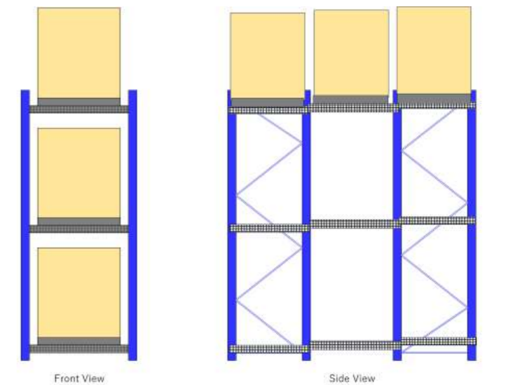
Push back rack design drawing 后推式货架设计图
