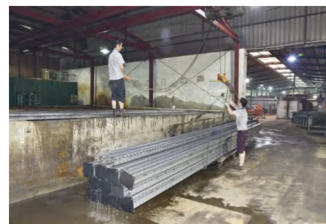
Pickling treatment 酸洗
