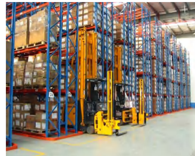
VNA rack project 窄巷式货架案例
