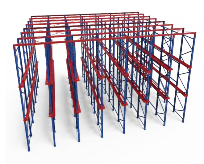
Drive-in rack project 驶入式货架案例
