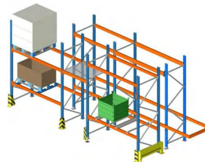
VNA 3D view 窄巷式货架3D效果图
